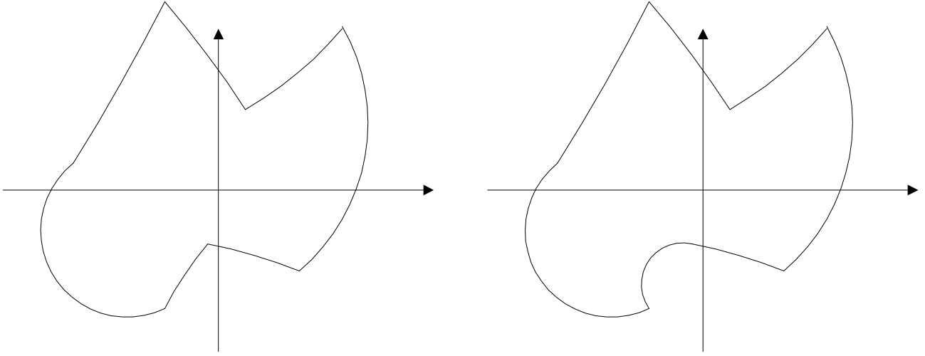
Figure 24: Star-shaped with center 0? Left: Yes. Right: No.
