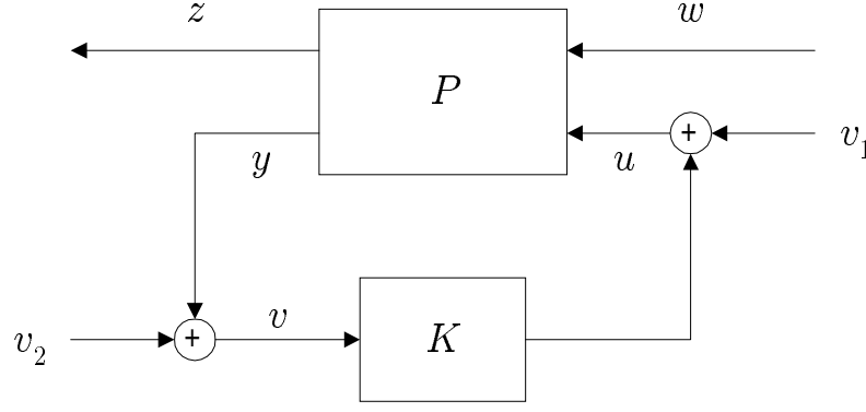
Figure 6: Interconnection to Test Stability
