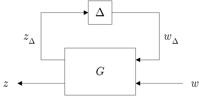
Figure 19: Uncertainty Pulled out of Component
