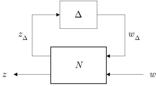
Figure 11: Uncertain closed-loop interconnection
