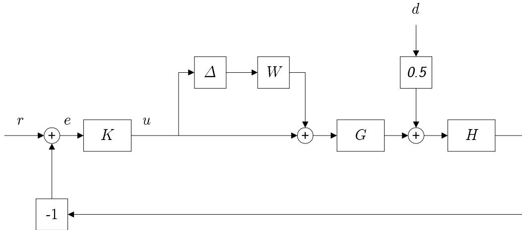
Figure 39: Tracking interconnection for exercise 2).
