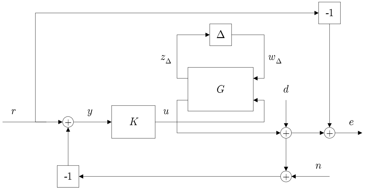
Figure 20: Uncertain closed-loop interconnection
