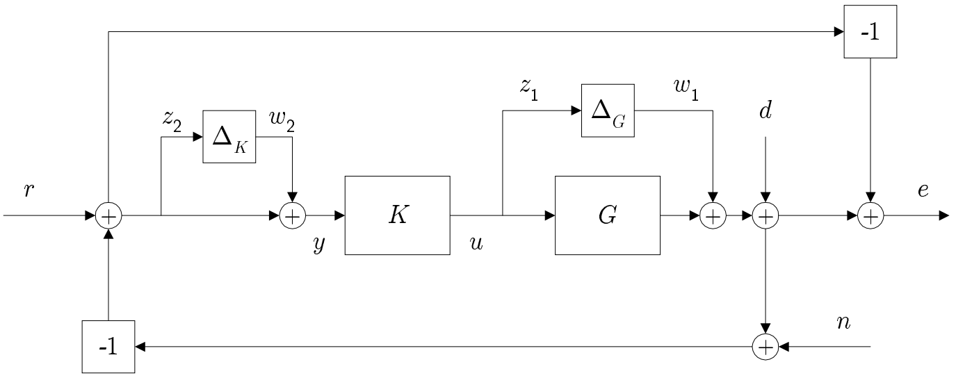
Figure 22: Uncertain closed-loop interconnection
