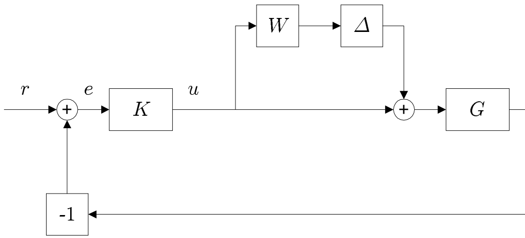
Figure 40: Tracking interconnection of simplified distillation column.
