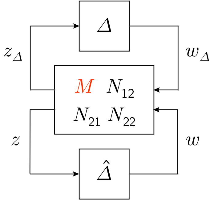
Figure 34: Equivalent Robust Stability Test
