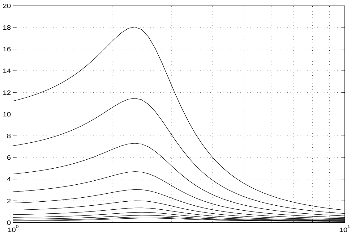
Figure 27: SSV of RM with r_1 = 1 , r_2 \in [0.1, 10] .
