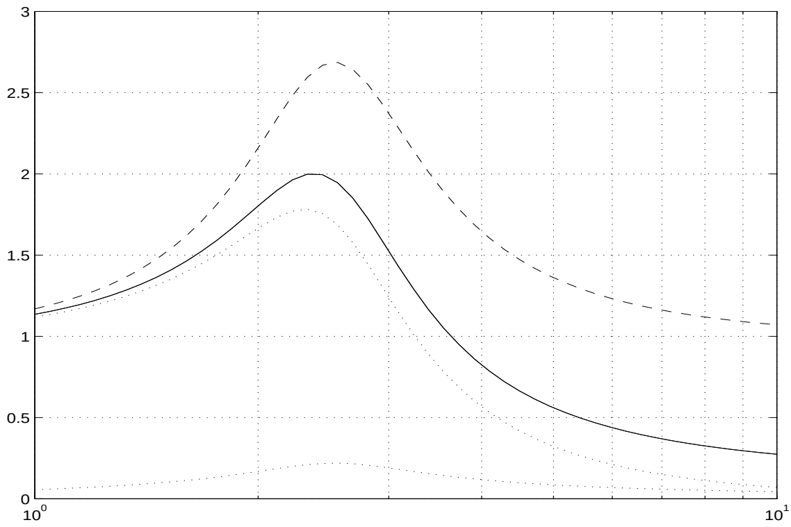
Figure 26: Magnitudes of M_{11} , M_{22} (dotted), norm of M (dashed), SSV of M (solid)
