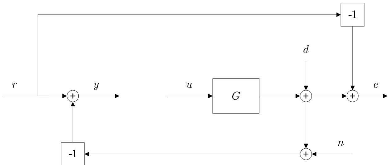
Figure 2: Open-loop interconnection that corresponds to Figure 1
