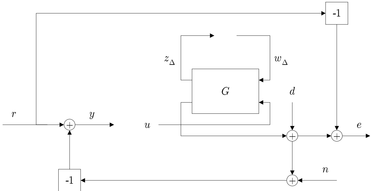
Figure 21: Uncertain open-loop interconnection
