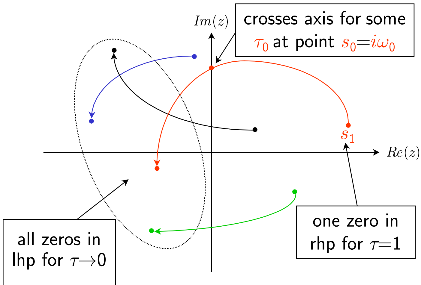
Figure 25: Movements of zeros
